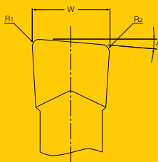
Width and Radius Modification with Right or Left Hand Lead Angle
