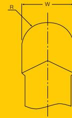
Radius Modification with Radial Grind for Undercutting
