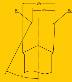
Left Hand with Angle and Radii
