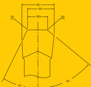
Width Modification with Two Angles
