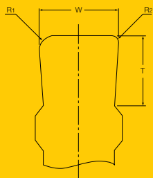
Width and Radius Mod with Limited Depth (Applies to <W> up to 2,47mm)
