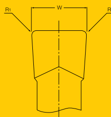
Width and Radius Modification with Radial Grind for Face Grooving
