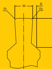
Width and Radius Modification with Break Corners for Chamfering
